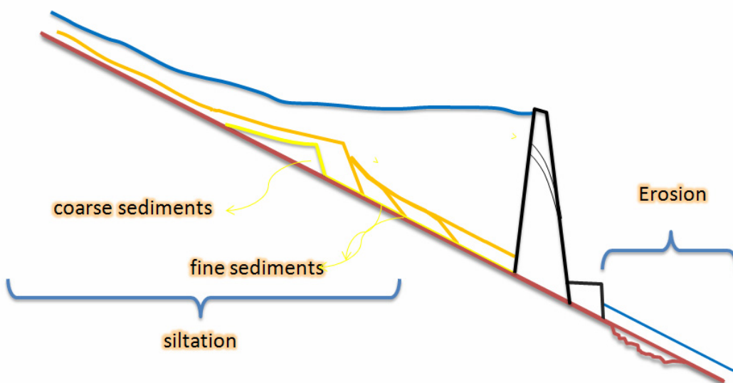
Figure 6 - Schematic drawing of the problems of sedimentation and erosion.
